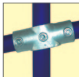
TYPE 219 2 SOCKET CROSS SIZES 2 - 4 ADJUSTABLE BETWEEN 0°-11°
