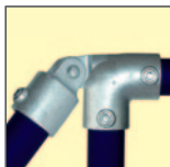
TYPE 175 SWIVEL STEP TEE SIZE 4 ONLY NB All swivel fittings are available as separate components
